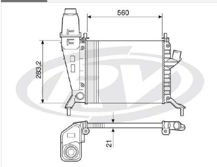
12580 GENERAL MOTORS
