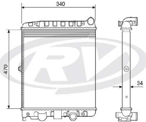
12509 VOLKSWAGEN
