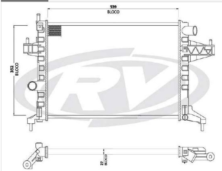
12578 GENERAL MOTORS
