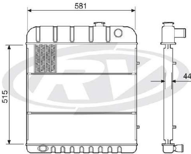
19212 GENERAL MOTORS
