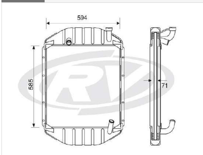
19106 MERCEDES - BENZ
