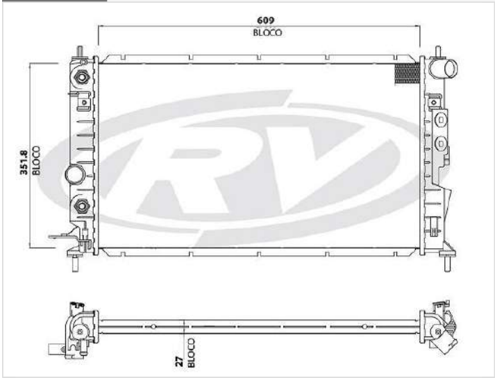
12571 GENERAL MOTORS
