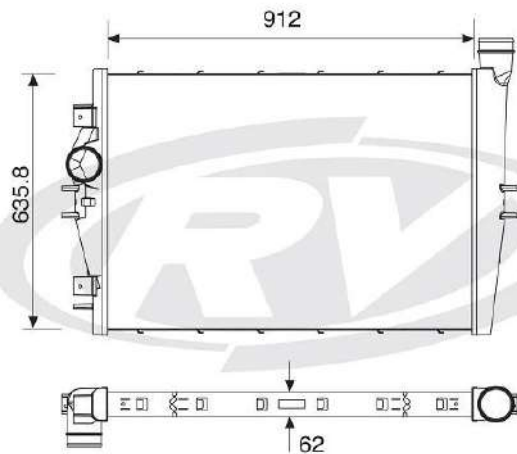
12677 MERCEDES - BENZ
