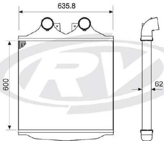
12692 MERCEDES - BENZ
