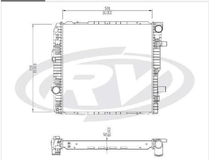
12005 MERCEDES - BENZ
