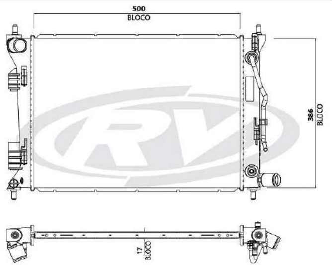
12702 HYUNDAI
