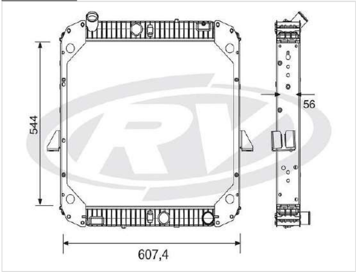
12029 MERCEDES - BENZ
