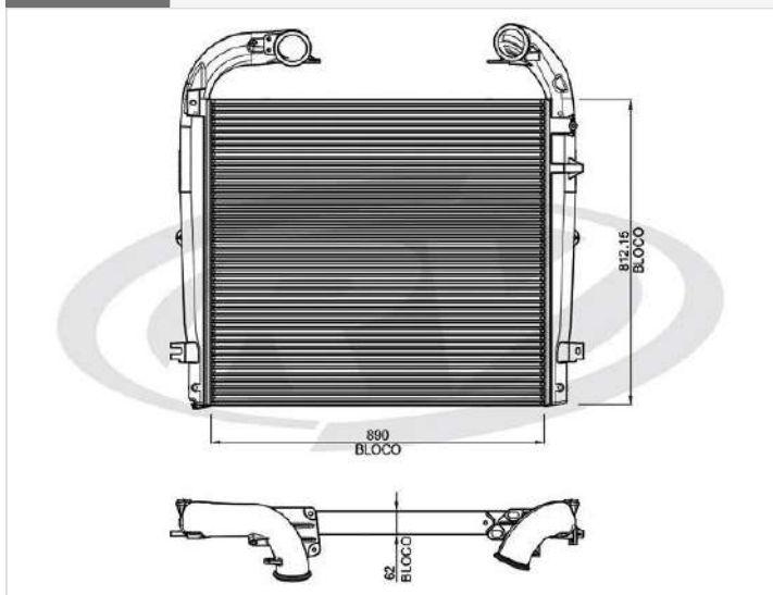
12650 SCANIA
